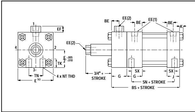
20B – Side Tapped Mount
