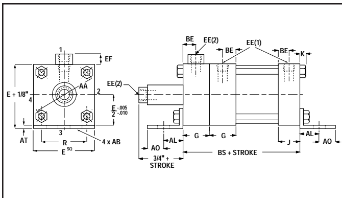
20Y – Angle Mount
