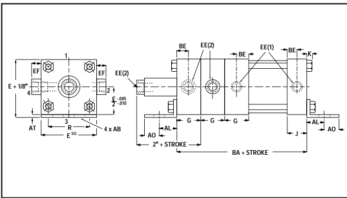
30Y – Angle Mount
