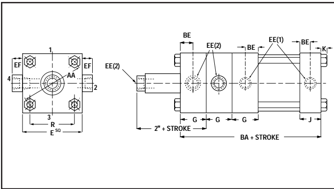
30K – No Mount
