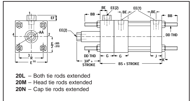
20L, M & N – Tie Rods Extended Mount
