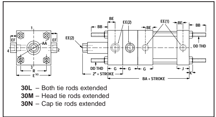
30L, M & N – Tie Rods Extended Mount
