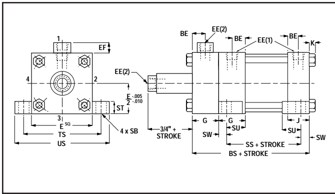
20A – Side Lugs Mount
