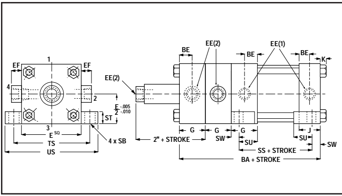
30A – Side Lugs Mount
