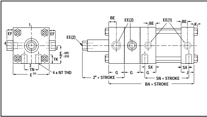
30B – Side Tapped Mount
